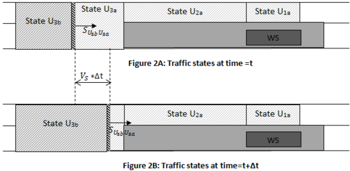
Figure 3-2: Position of The Shockwave S_{U_{3b}U_{3a}} at A) Time t and B) Time t+\Delta t
