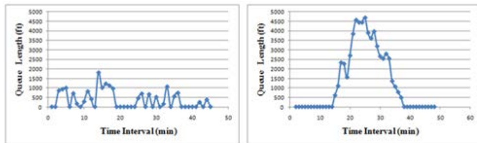
Figure 1-1: Queue Length for A) Intermittent Queue B) Moving Queue
